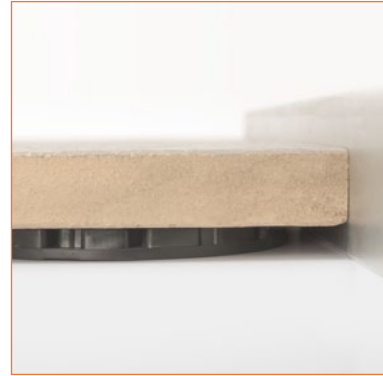
At the edge and in the corners you fit Standard-Pads with no joint bars.
